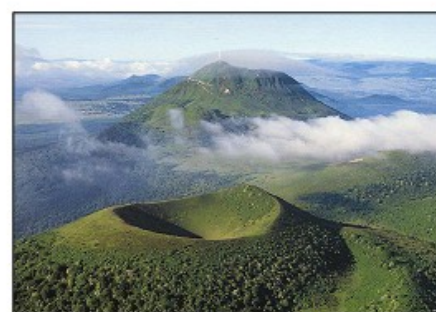
Volcanoes of Auvergne
